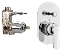
5 - Way (3 inlets + 2 outlets) single lever concealed diverter Exposed part F1018711 ₹ 2,835 Concealed Part F4020101 ₹ 4,750 Set ₹ 7,585
